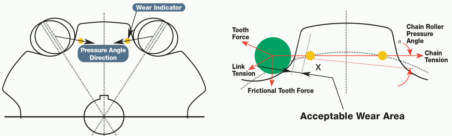
Figure 1 – Theory of Operation
